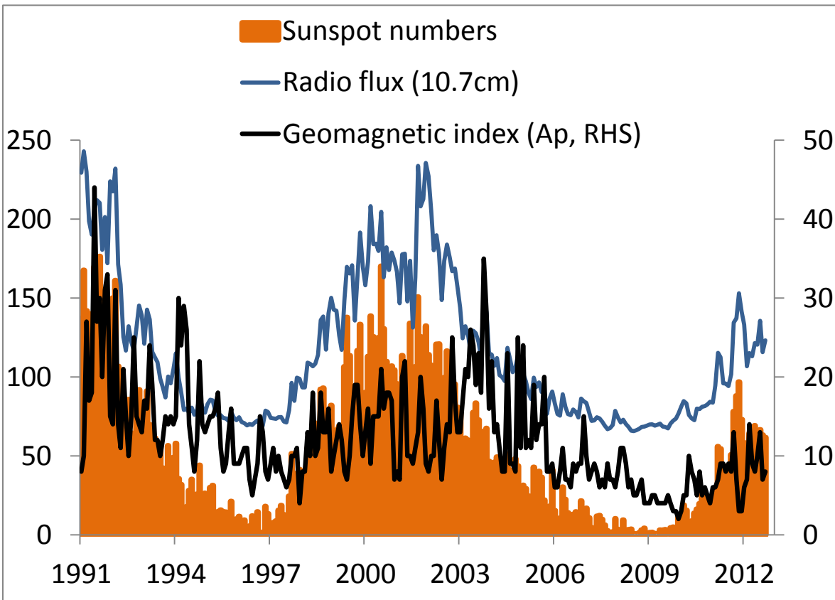
Figure #. Solar and Geomagnetic Activity Indices, Actual and Smoothed, 1991-2012
